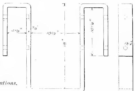
Figs. 4802-4803. SPRING-HANGER.
